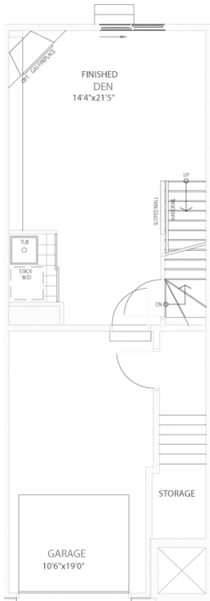
GROUND FLOOR PLAN 335 SQ.FT.
