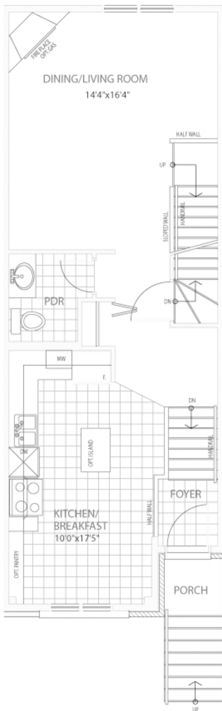
MAIN (SECOND) FLOOR PLAN 615 SQ.FT.
