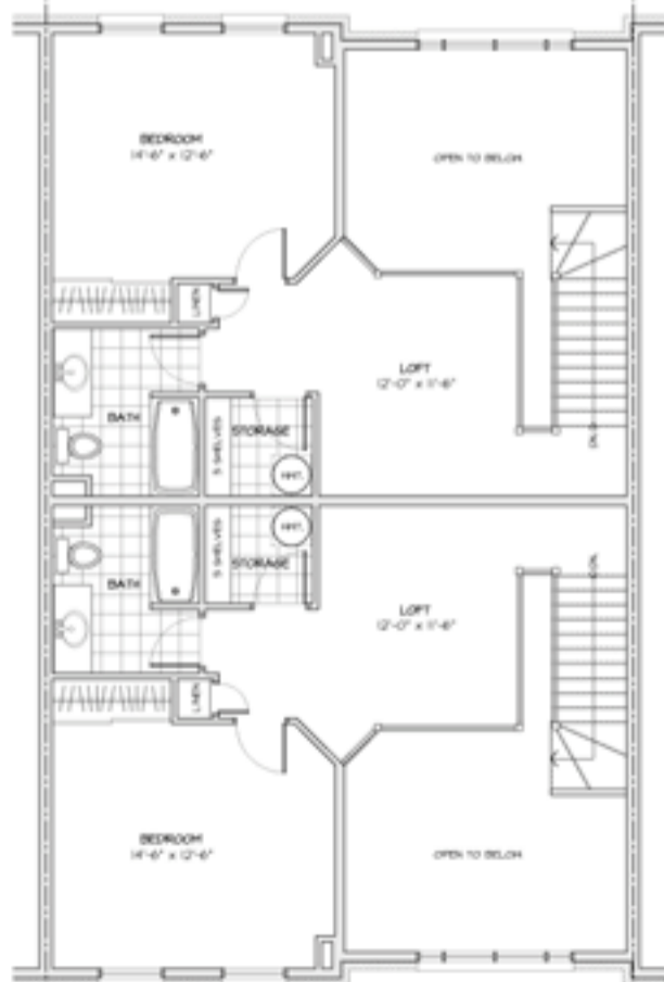
THIRD FLOOR PLAN EACH SITE - 350 sq. ft. + 175 sq. ft. OPEN TO BELOW TOTAL FLOOR - 110 sq. ft. + 350 sq. ft. OPEN TO BELOW
