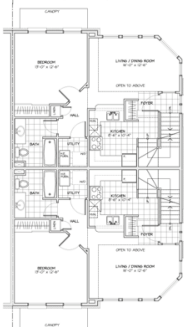
SECOND FLOOR PLAN EACH SITE - 125 sq. ft. TOTAL FLOOR - 1450 sq. ft.
